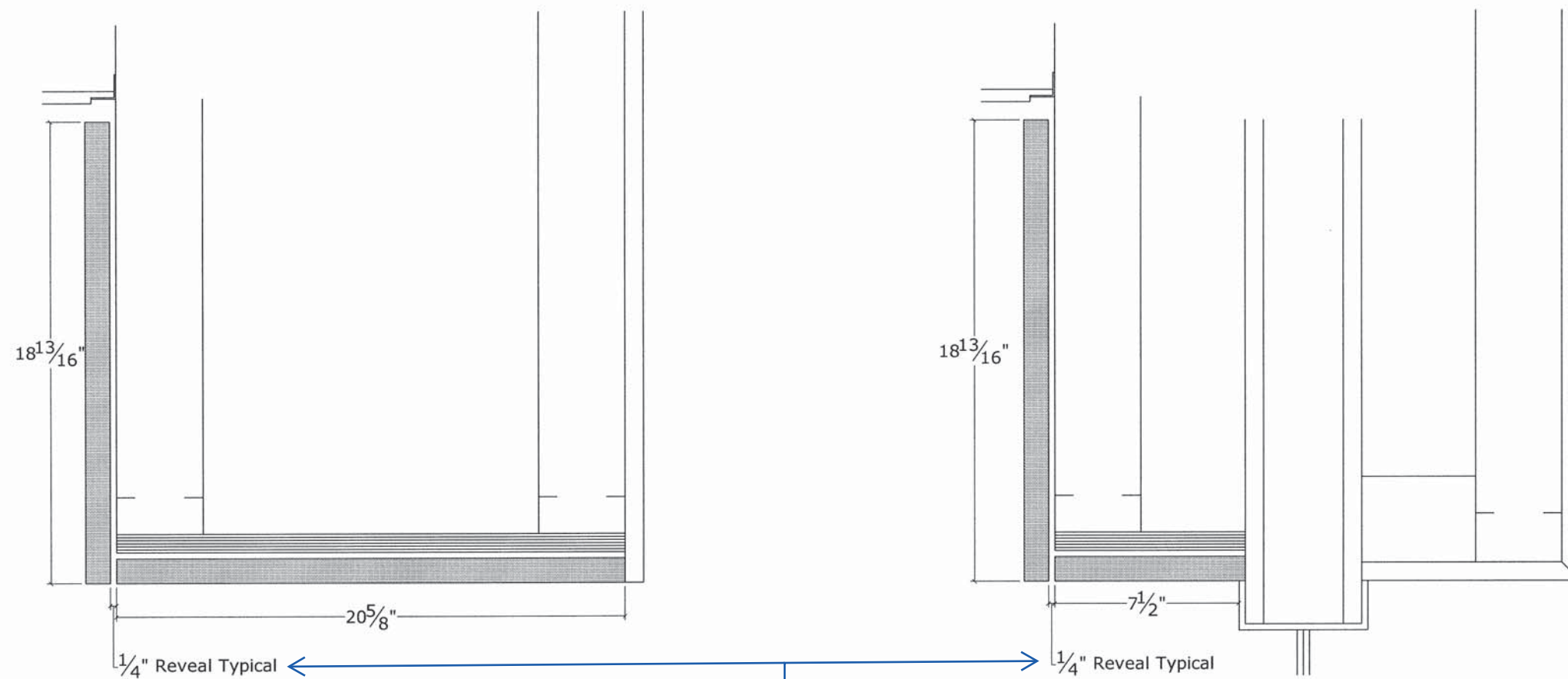
Section View Soffit 1 5 SCALE: No Scale
