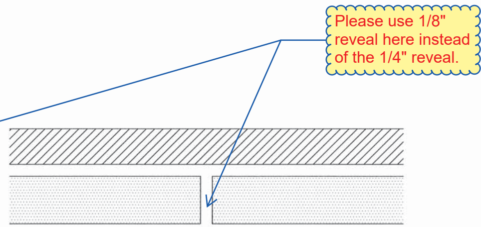
2 6 Typical Detail Butt Joint SCALE: No Scale
